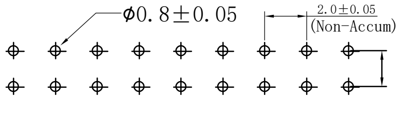
PCB Layout
