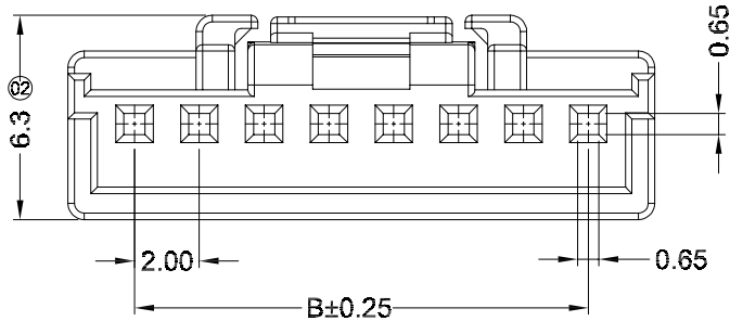
05P~15P Shape Scale 1:1
