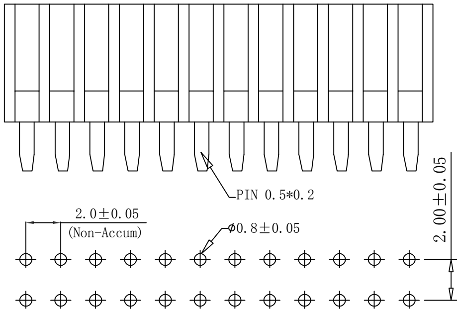
PCB Layout
