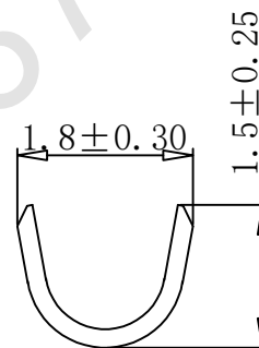
b-b SECTION
