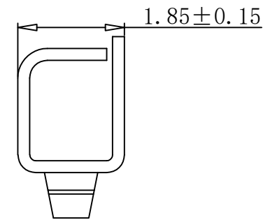
c-c SECTION
