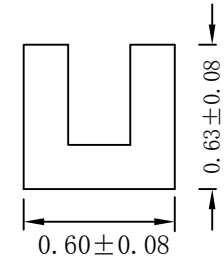
C-C SECTION
