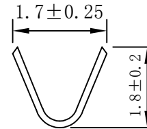
B-B SECTION
