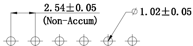
PCB LAYOUT
