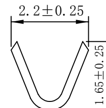
b-b SECTION
