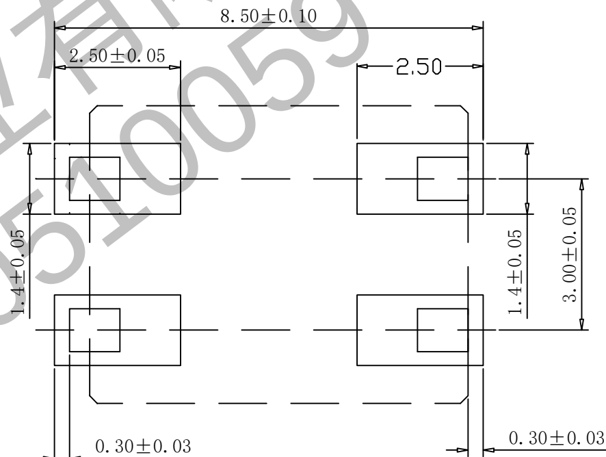
PCB LAYOUT
